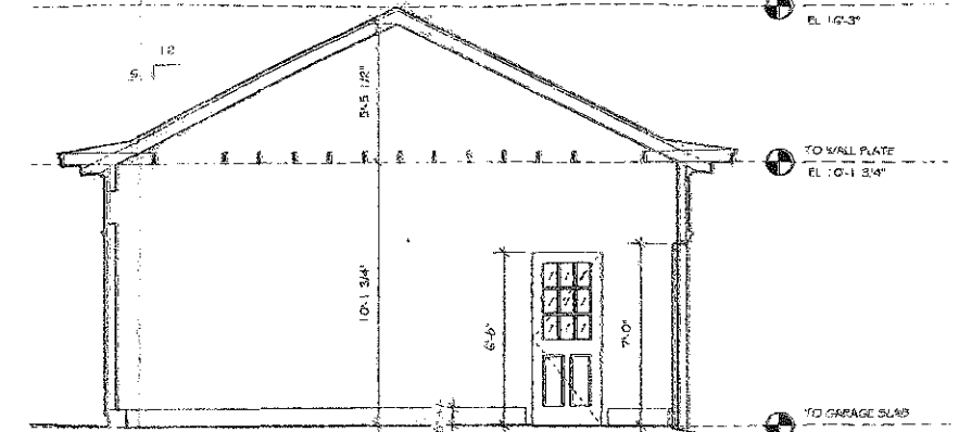
2 EXISTING GARAGE SECTION SCALE 1/4" = 1'-0"
