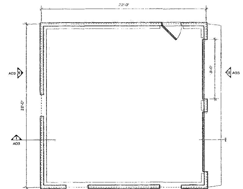
1 EXISTING GARAGE PLAN SCALE 1/4" = 1'-0"
